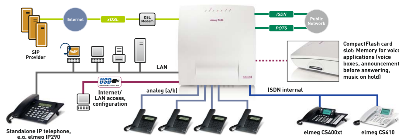
Example of elmeg T484 configuration (includes optional equipment)
